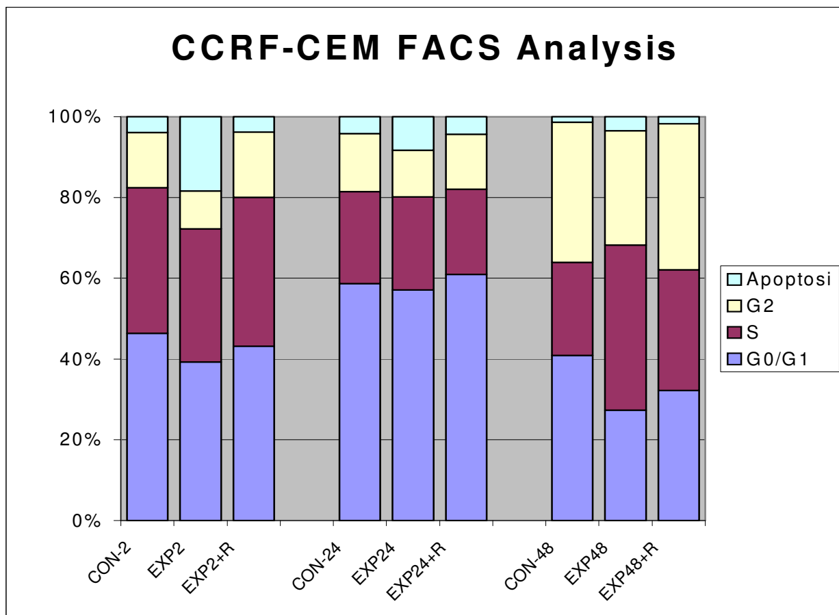
Fig. 5: GRAPH OF RESULTS OF FACS ANALYSIS CEM leucemic cells exposed to electromagnetic field. The sections of the columns represent the percentages in the G0/G1, S, G2/M and apoptosis phases of the cell cycle.
