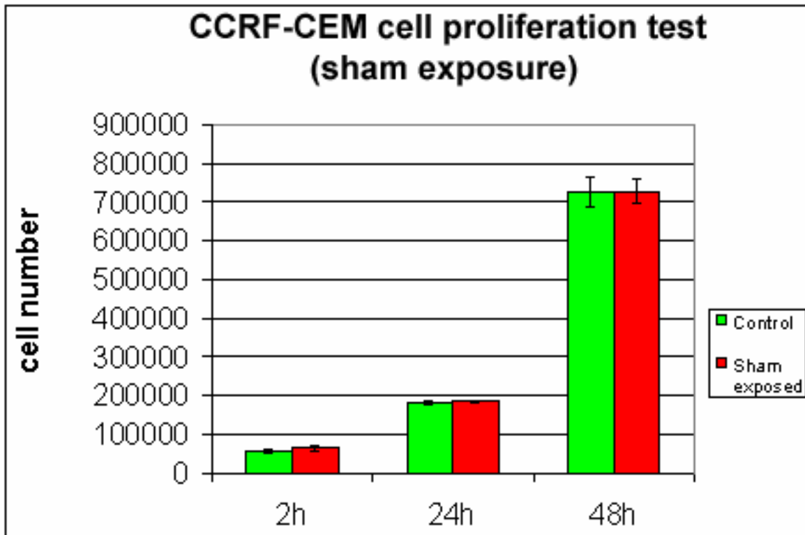
Fig. 3: Graph showing cell proliferation in CCRF-CEM T leucemic cell cultures. Sham exposure: the cells cultivated under experimental conditions but without electromagnetic field do not display any significant difference to the proliferation test.
